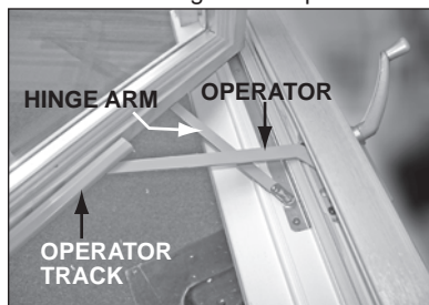
FIGURE 5 – Single-Arm Operator
