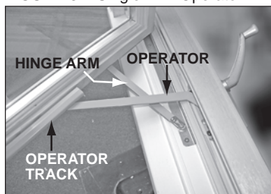
FIGURE 3 – Single-Arm Operator
