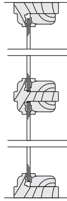
Single Glazed 1-3/8" TDL A
