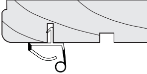
#13 ) Side Inside Stop Complete with Weather Strip
