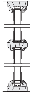
3/4" Insul 7/8" TDL B & D
