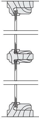
Single Glazed 7/8" TDL A & C
