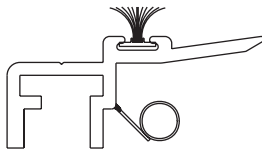
#11 & 12) Vinyl Interlock with Weather Strip Extrusion #6014-V
