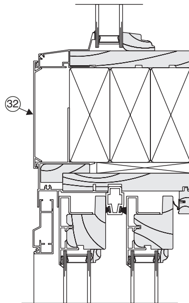
Aluma TFT 3 1/2" Horizontal Spread Mull
