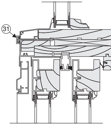
Aluma TFT Tight Horizontal Mull
