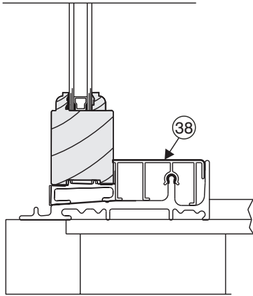
Poly/Prime Insert with Brick Mould
