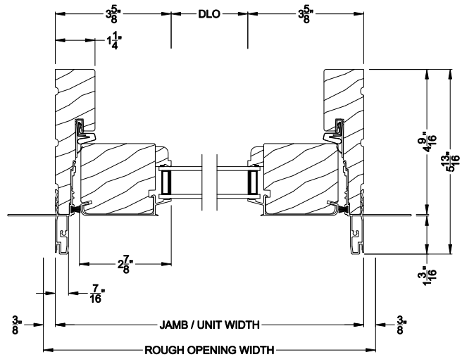
PREMIUM OUTSWING SIDELITE (8611) Horizontal Section - 2-1/4" Panel
