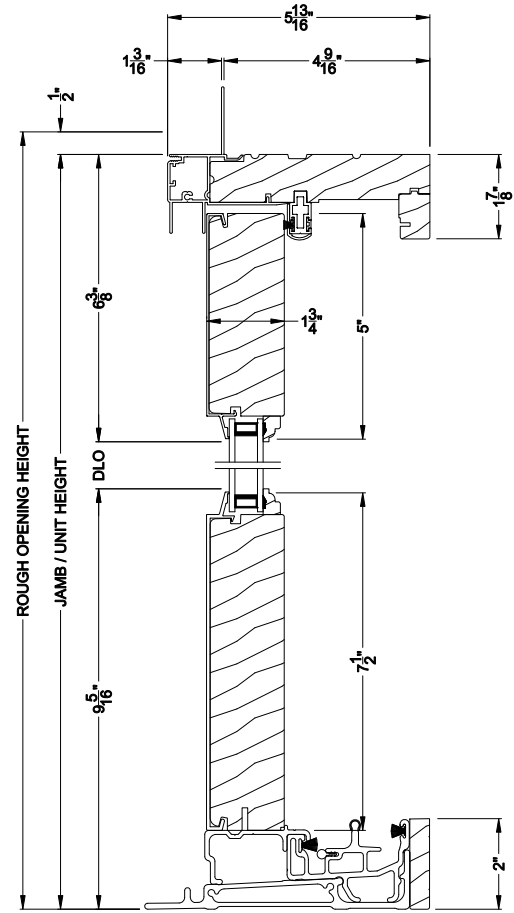
PREMIUM FRENCH SLIDING PATIO DOOR (8715) Vertical Section - Fixed Sidelite with Low profile sill stop
