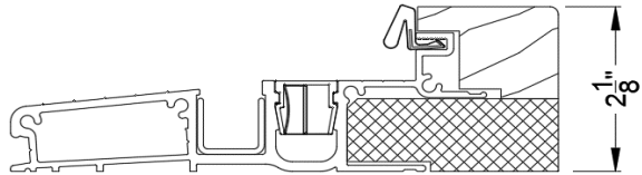
Standard Sill
