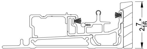
Standard Sill
