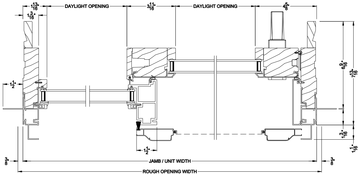
CONTEMPORARY SLIDING PATIO DOOR WITH DIRECT-SET (8723) Horizontal Section - 2 Panel Equal or Picture Slider - 6-9/16" jamb
