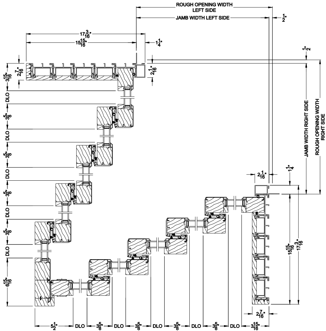
CONTEMPORARY 2-1/4" MULTI-SLIDE PATIO DOOR (8726) Horizontal Section - 5L5R Panel Inside Corner Door
